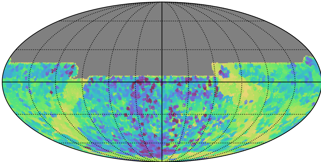
weather_cloudso12v3.4_10yrs All sky y band: Min skyBrightness
