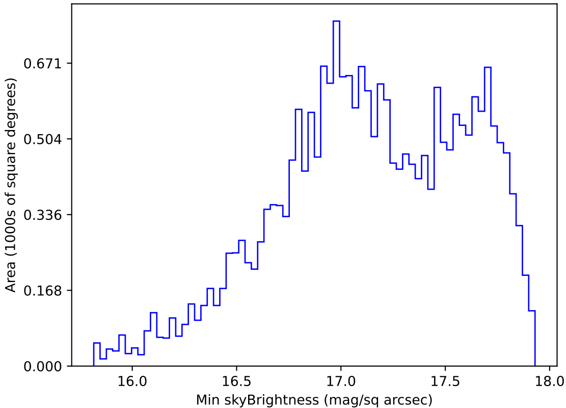
weather_cloudso12v3.4_10yrs All sky y band: Min skyBrightness
