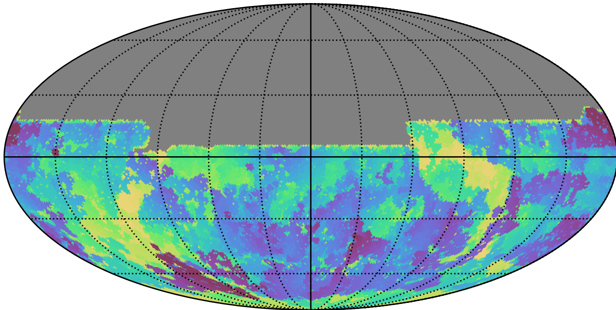
weather_cloudso12v3.4_10yrs All sky u band: Min skyBrightness
