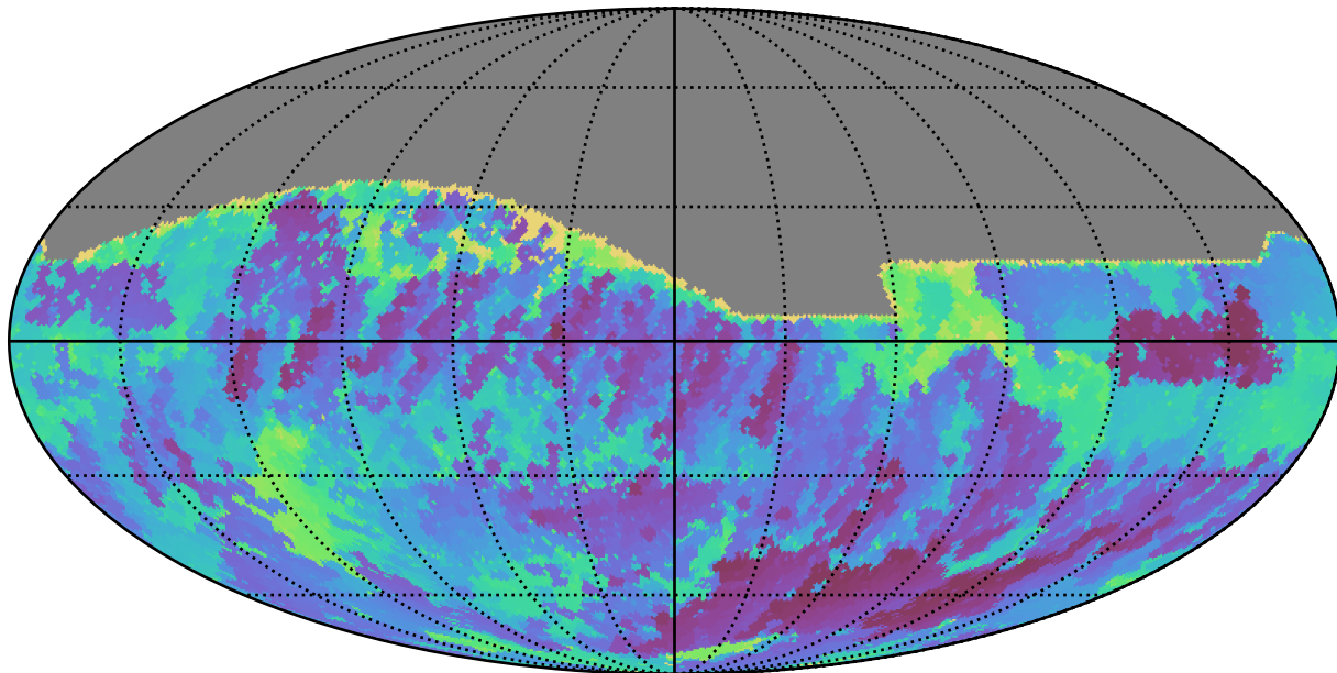
weather_cloudso12v3.4_10yrs All sky r band: Min skyBrightness
