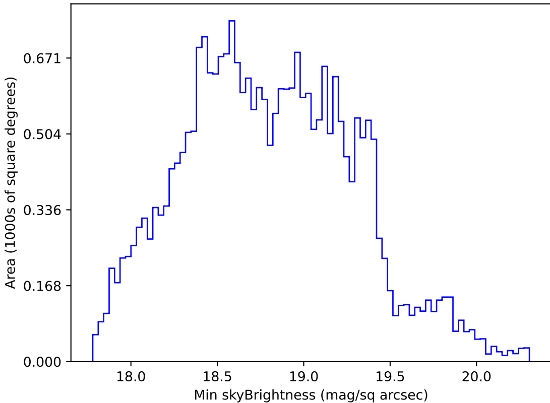
weather_cloudso12v3.4_10yrs All sky r band: Min skyBrightness
