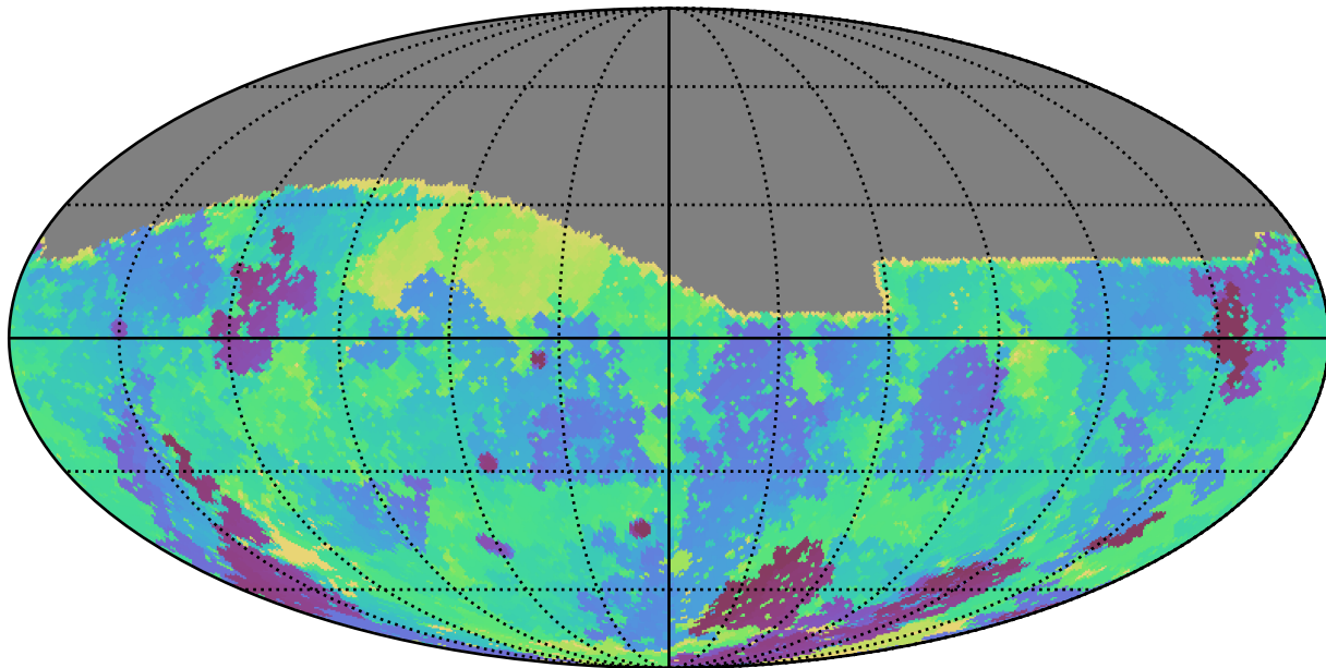
weather_cloudso12v3.4_10yrs All sky g band: Min skyBrightness
