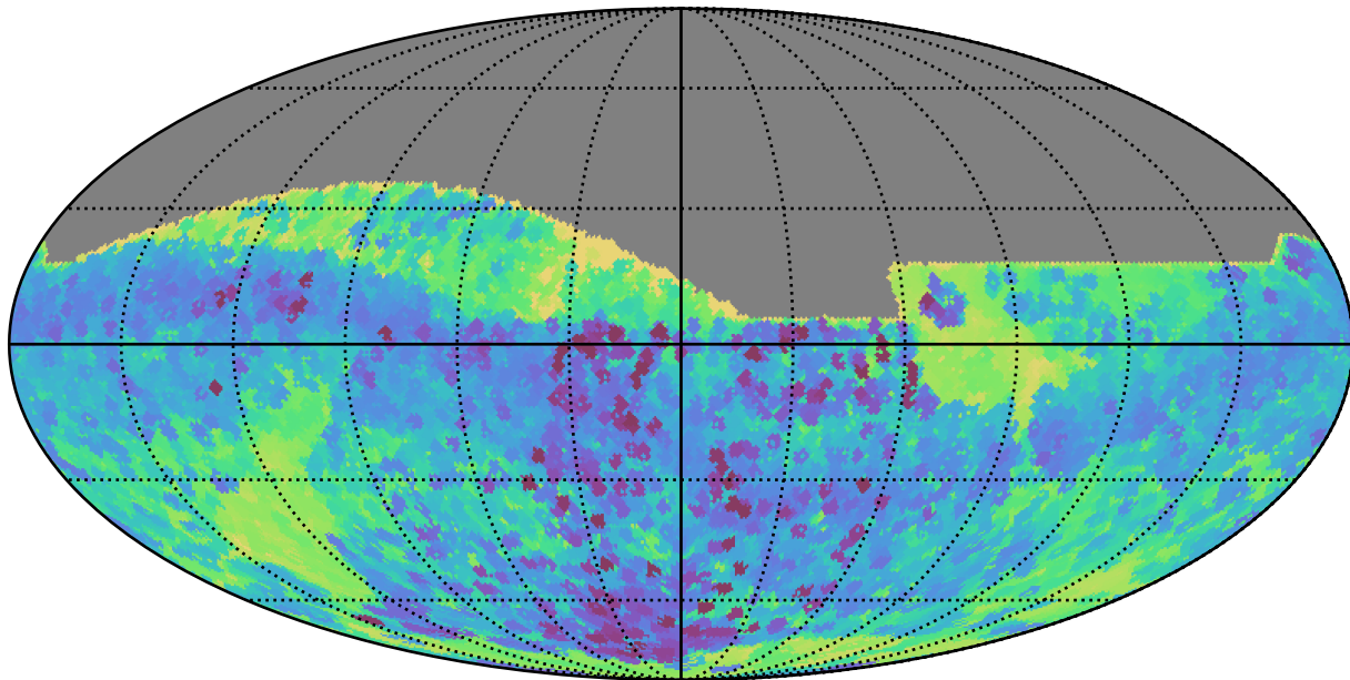
weather_cloudso12v3.4_10yrs All sky all bands: Min skyBrightness
