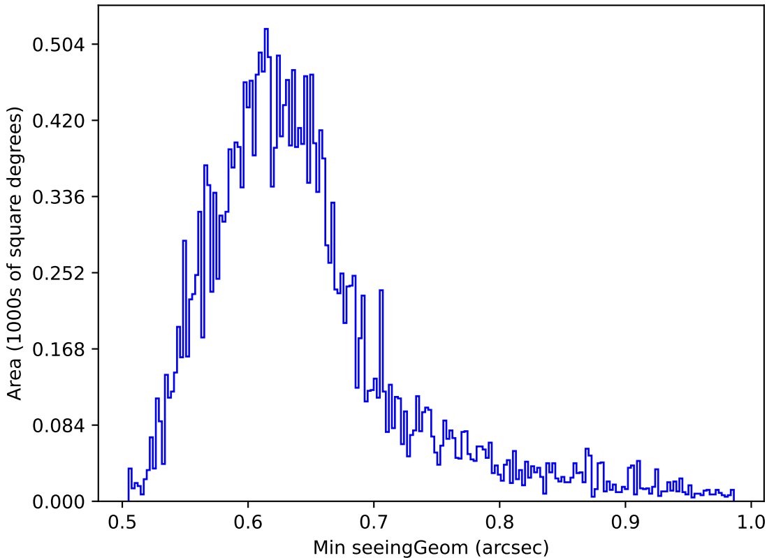
weather_cloudso12v3.4_10yrs Yr 1 z band: Min seeingGeom
