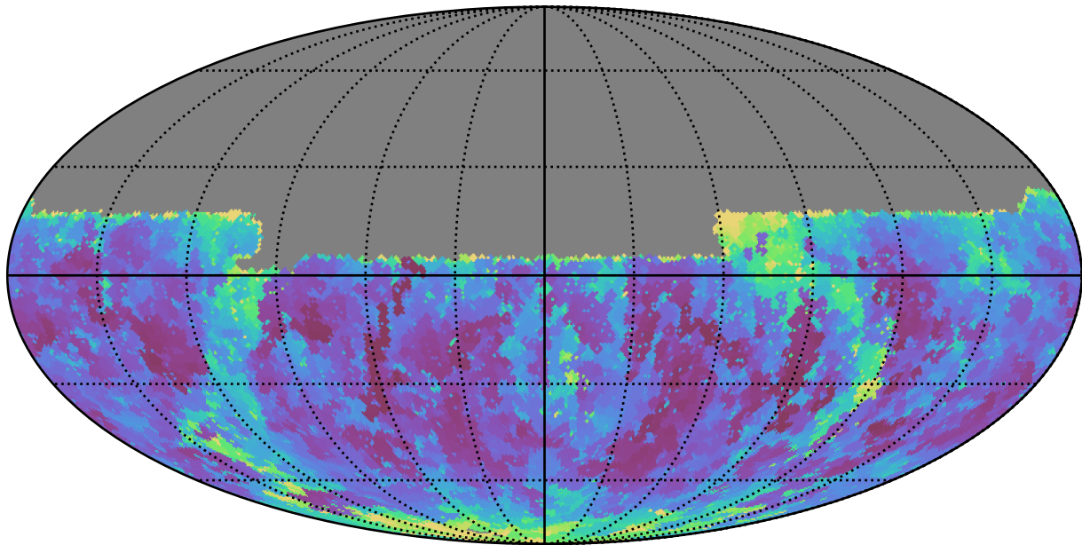
weather_cloudso12v3.4_10yrs Yr 1 y band: Min seeingGeom
