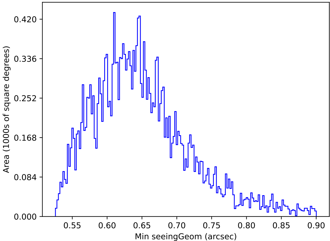
weather_cloudso12v3.4_10yrs Yr 1 y band: Min seeingGeom
