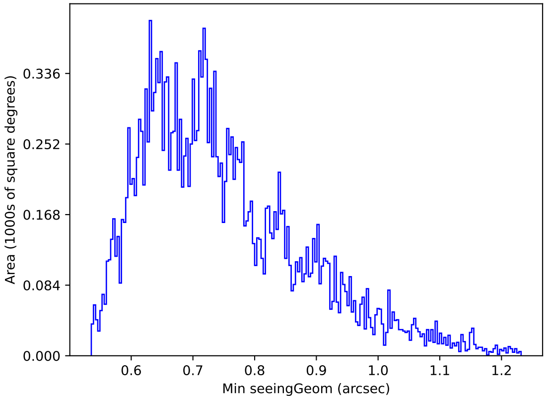
weather_cloudso12v3.4_10yrs Yr 1 u band: Min seeingGeom
