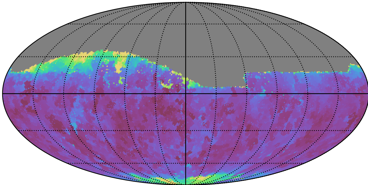
weather_cloudso12v3.4_10yrs Yr 1 r band: Min seeingGeom
