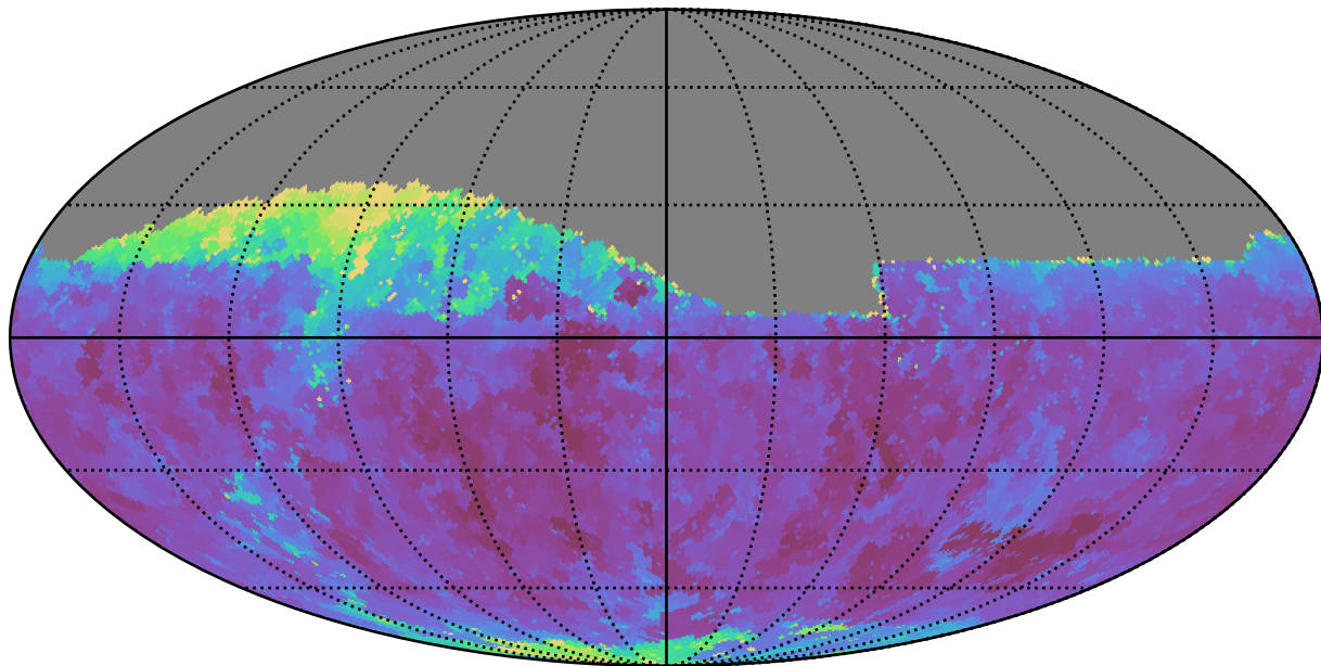
weather_cloudso12v3.4_10yrs Yr 1 i band: Min seeingGeom
