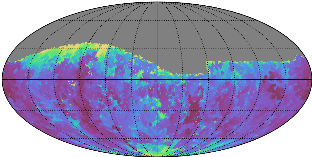
weather_cloudso12v3.4_10yrs Yr 1 g band: Min seeingGeom
