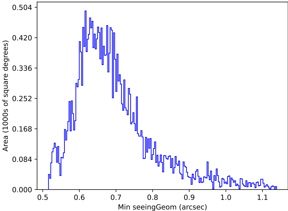
weather_cloudso12v3.4_10yrs Yr 1 g band: Min seeingGeom
