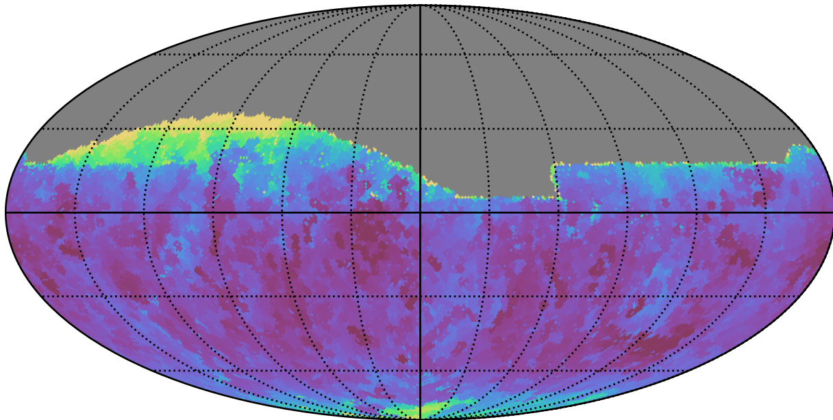
weather_cloudso12v3.4_10yrs Yr 1 all bands: Min seeingGeom
