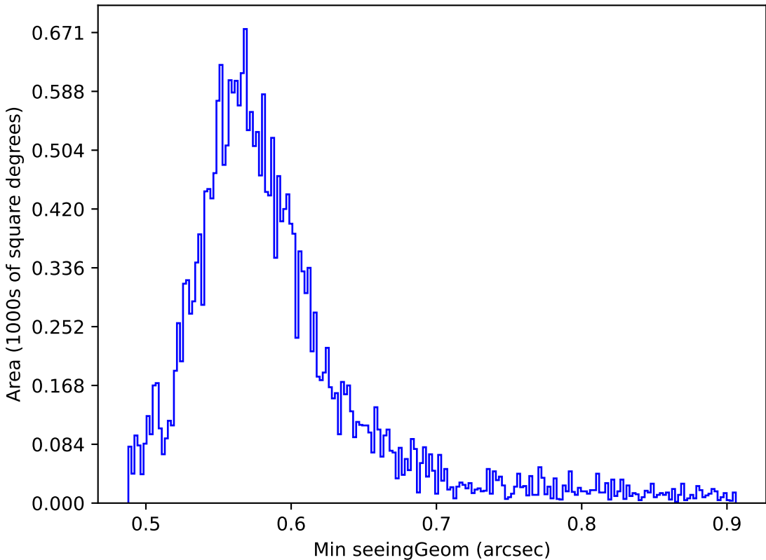
weather_cloudso12v3.4_10yrs Yr 1 all bands: Min seeingGeom
