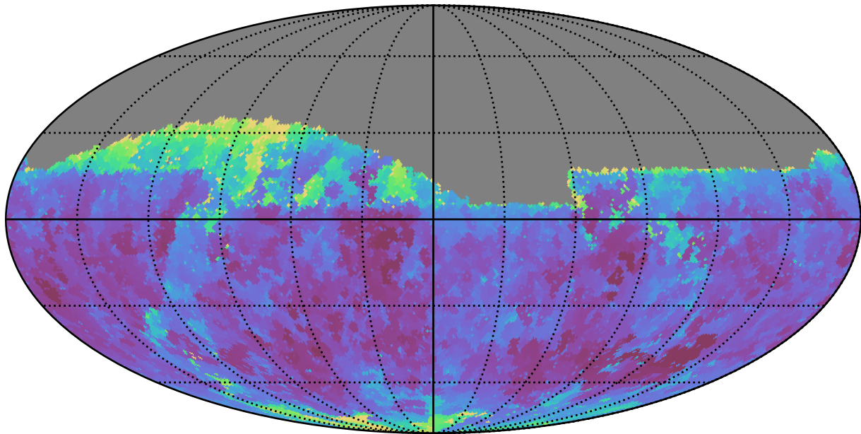
weather_cloudso12v3.4_10yrs Yr 1 z band: Min seeingEff
