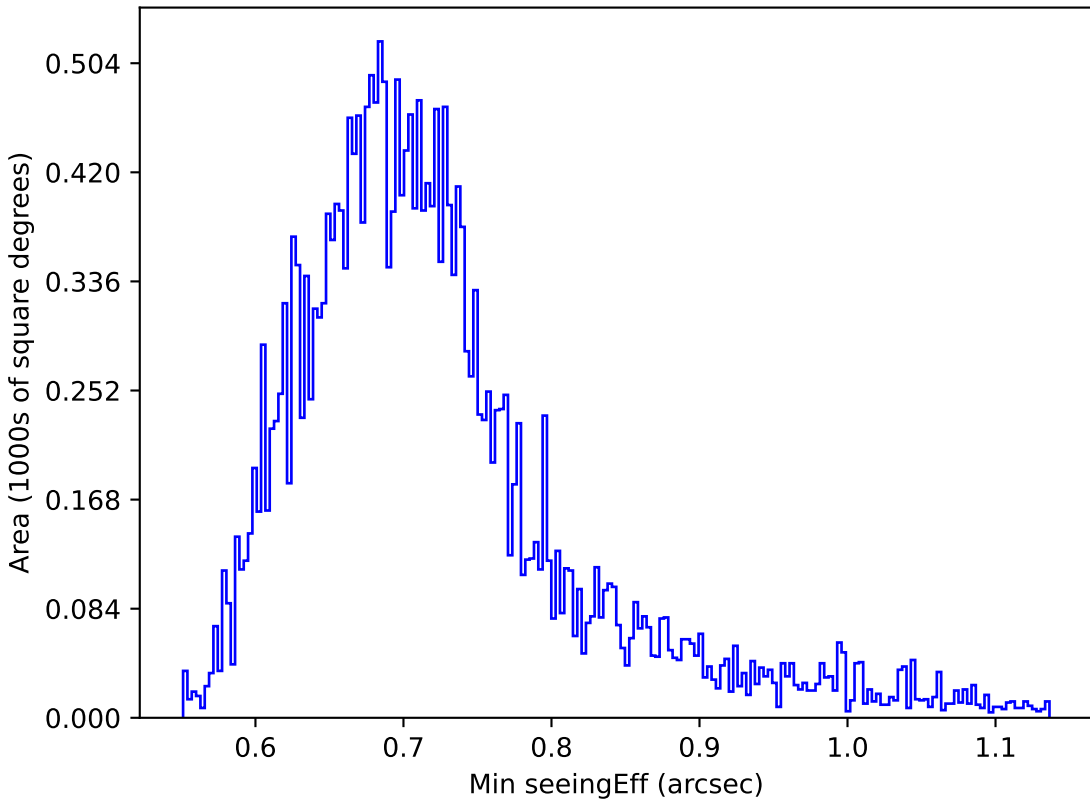
weather_cloudso12v3.4_10yrs Yr 1 z band: Min seeingEff
