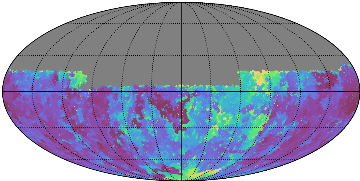
weather_cloudso12v3.4_10yrs Yr 1 u band: Min seeingEff
