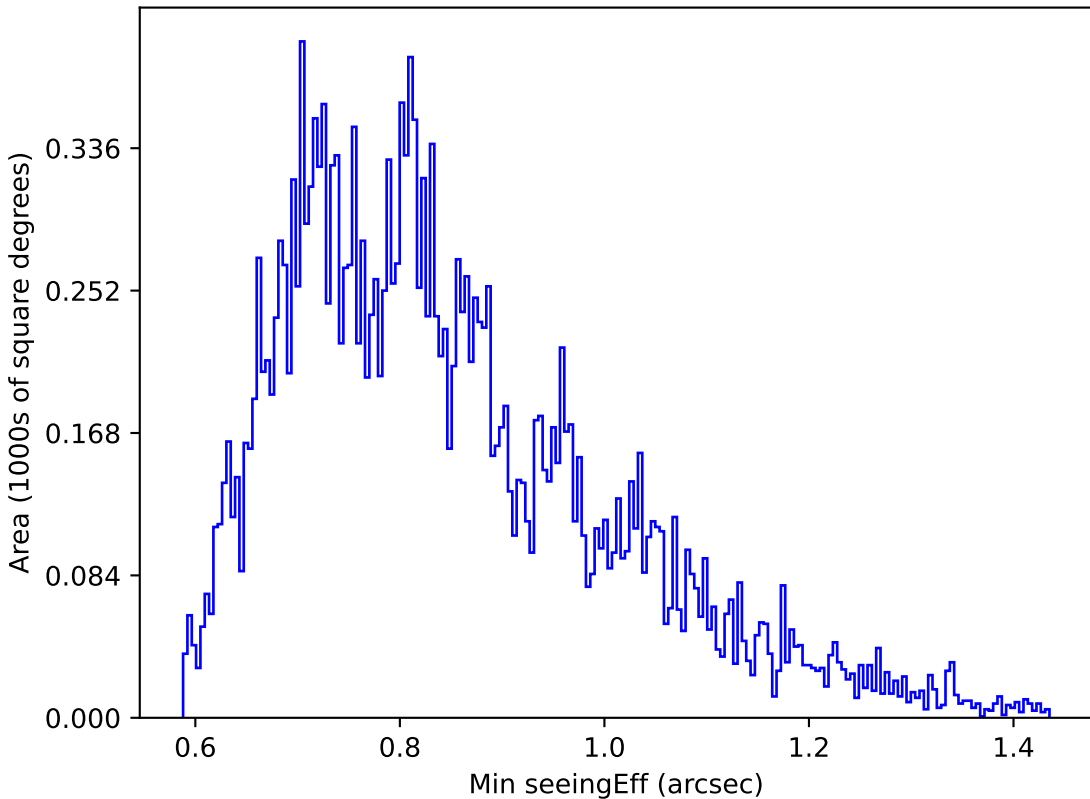
weather_cloudso12v3.4_10yrs Yr 1 u band: Min seeingEff
