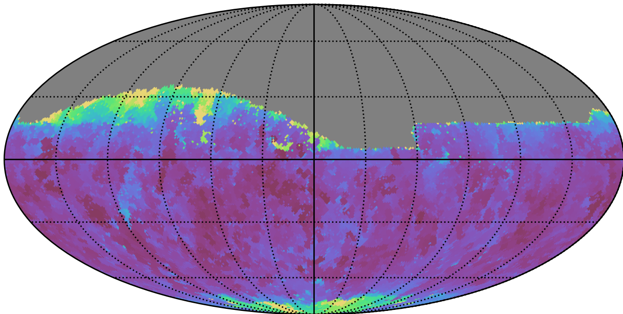
weather_cloudso12v3.4_10yrs Yr 1 r band: Min seeingEff
