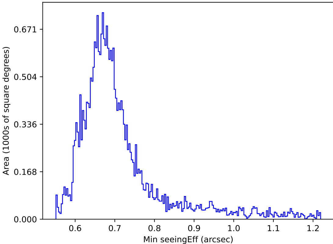
weather_cloudso12v3.4_10yrs Yr 1 i band: Min seeingEff
