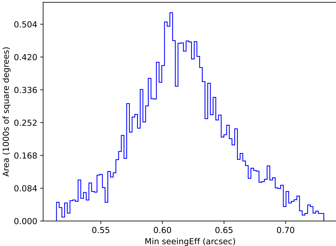
weather_cloudso12v3.4_10yrs WFD z band: Min seeingEff
