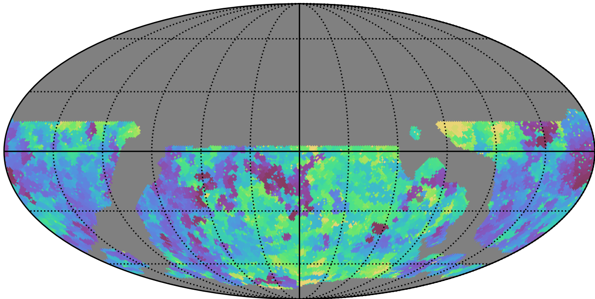
weather_cloudso12v3.4_10yrs WFD u band: Min seeingEff
