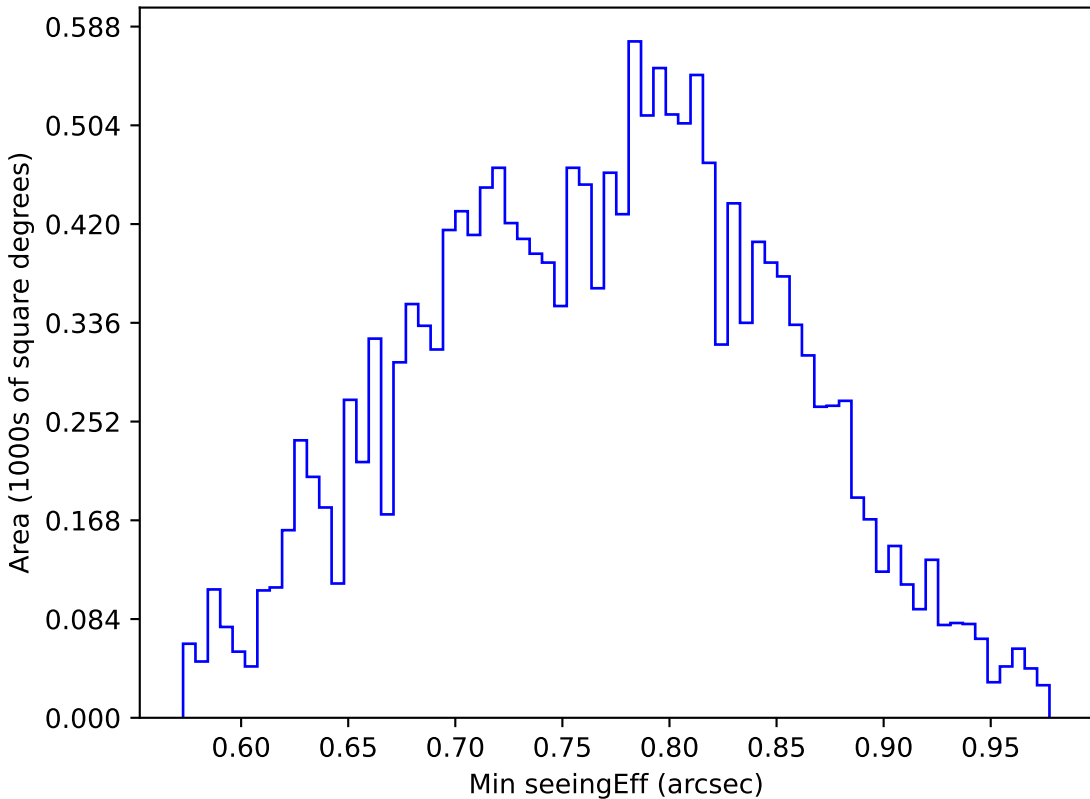
weather_cloudso12v3.4_10yrs WFD u band: Min seeingEff
