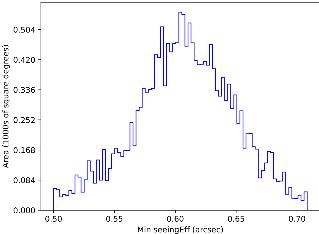
weather_cloudso12v3.4_10yrs WFD i band: Min seeingEff
