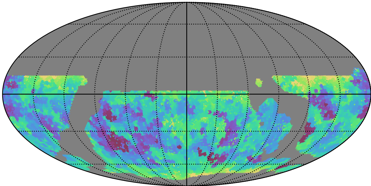
weather_cloudso12v3.4_10yrs WFD g band: Min seeingEff
