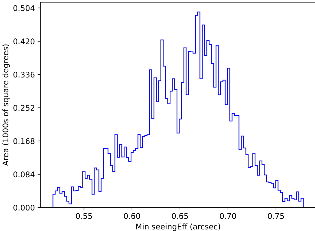
weather_cloudso12v3.4_10yrs WFD g band: Min seeingEff
