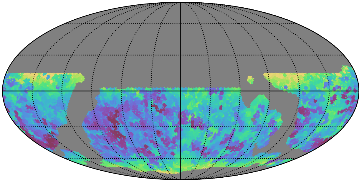
weather_cloudso12v3.4_10yrs WFD all bands: Min seeingEff
