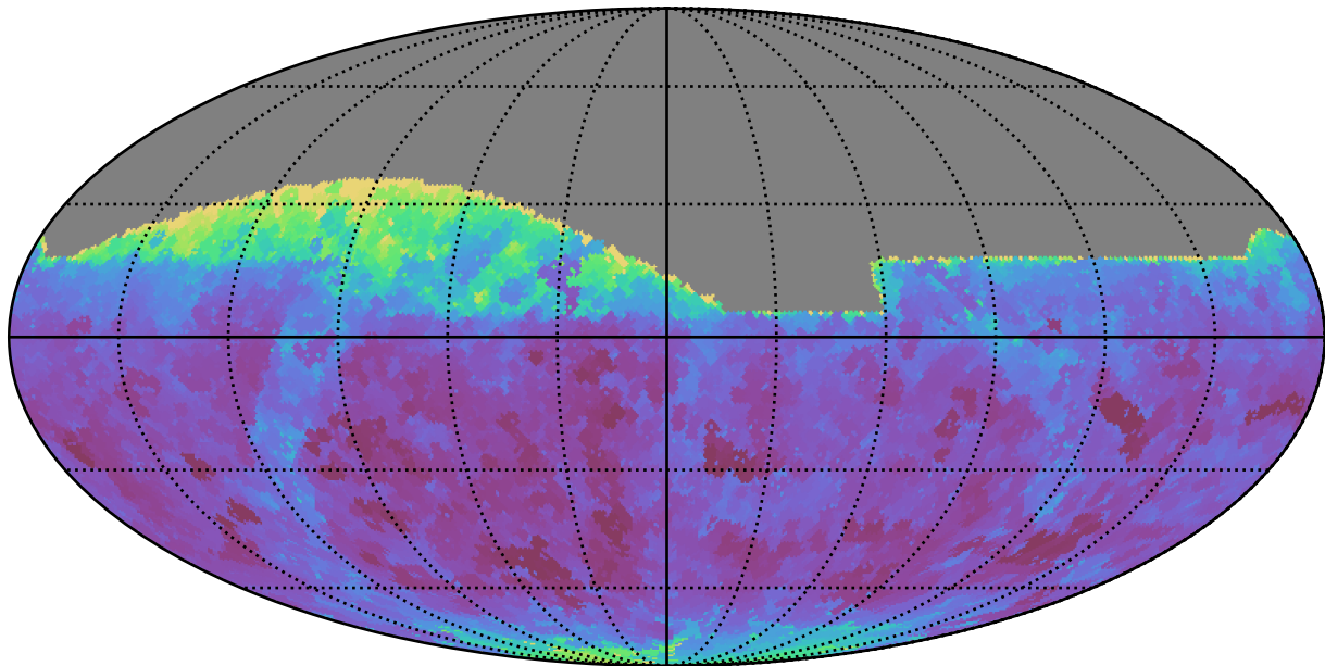
weather_cloudso12v3.4_10yrs All sky z band: Min seeingEff
