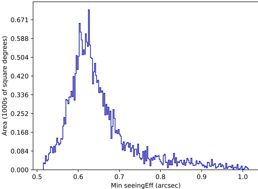
weather_cloudso12v3.4_10yrs All sky z band: Min seeingEff
