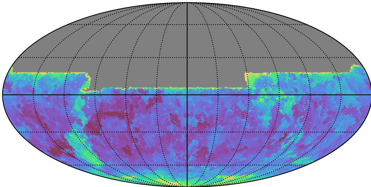
weather_cloudso12v3.4_10yrs All sky y band: Min seeingEff
