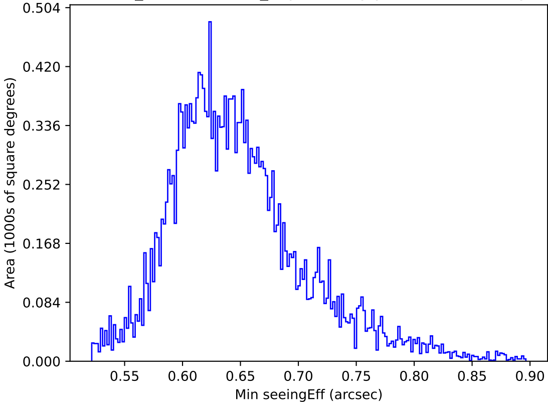
weather_cloudso12v3.4_10yrs All sky y band: Min seeingEff
