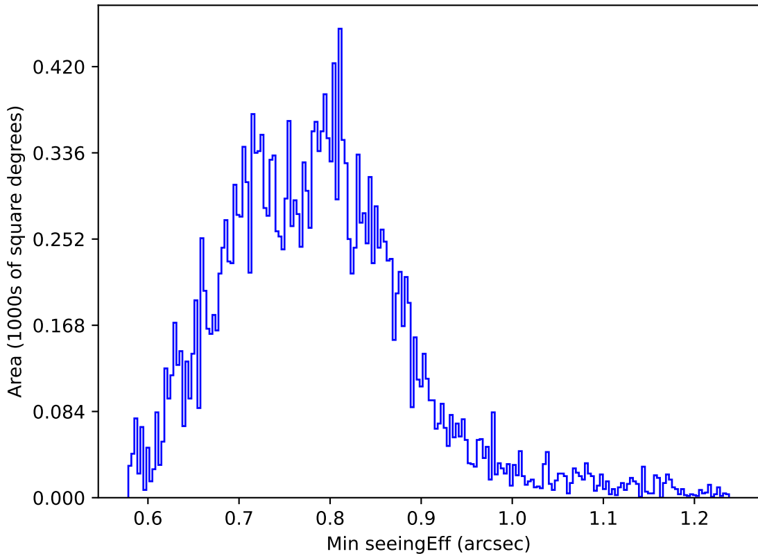
weather_cloudso12v3.4_10yrs All sky u band: Min seeingEff
