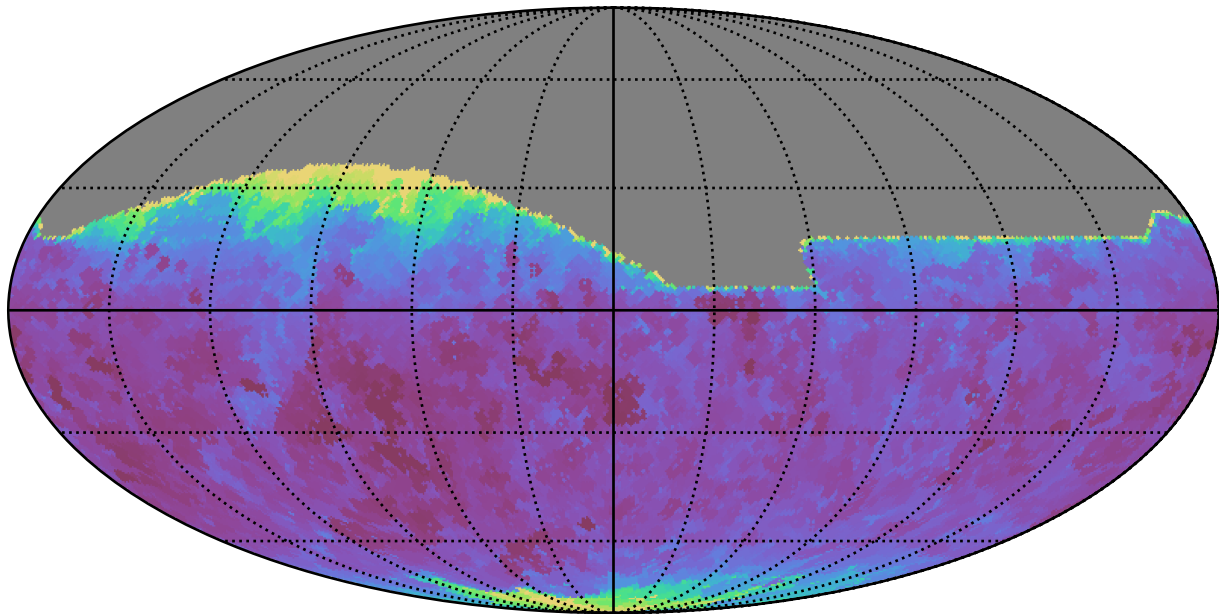
weather_cloudso12v3.4_10yrs All sky r band: Min seeingEff
