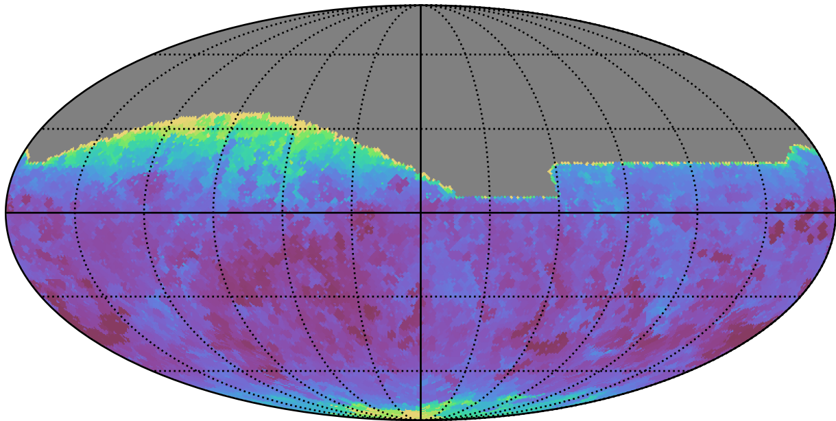
weather_cloudso12v3.4_10yrs All sky i band: Min seeingEff
