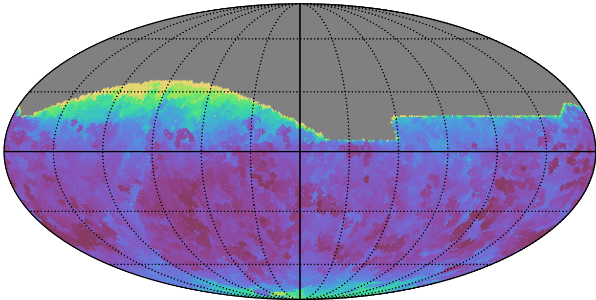
weather_cloudso12v3.4_10yrs All sky all bands: Min seeingEff
