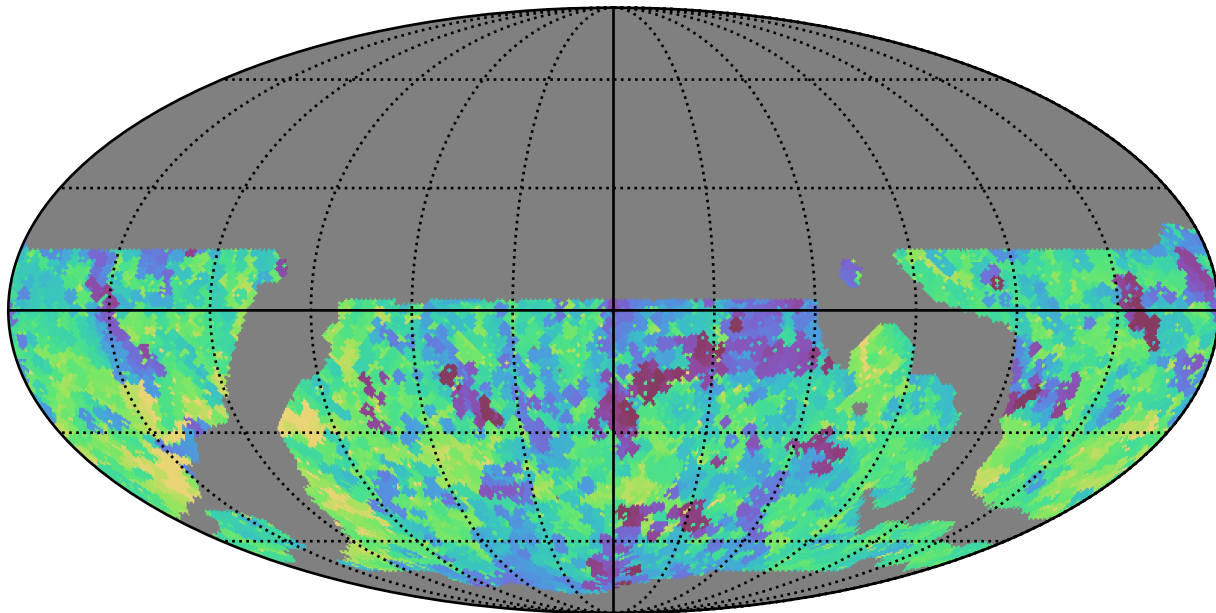
weather_cloudso12v3.4_10yrs WFD z band: Min saturation_mag
