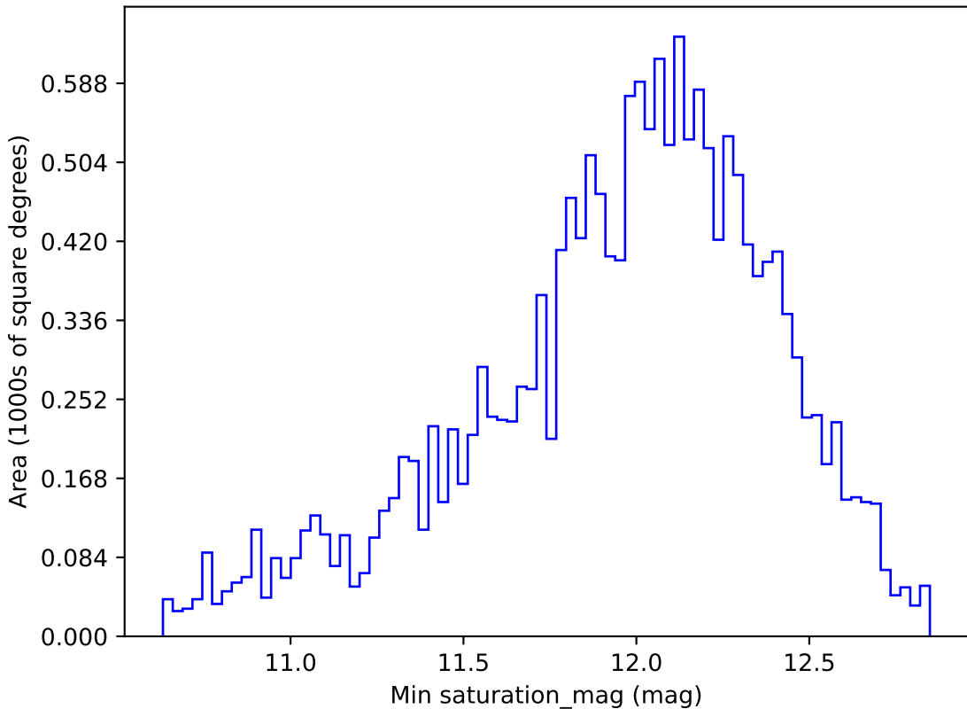
weather_cloudso12v3.4_10yrs WFD z band: Min saturation_mag
