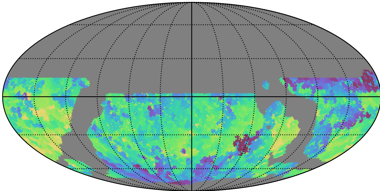
weather_cloudso12v3.4_10yrs WFD u band: Min saturation_mag
