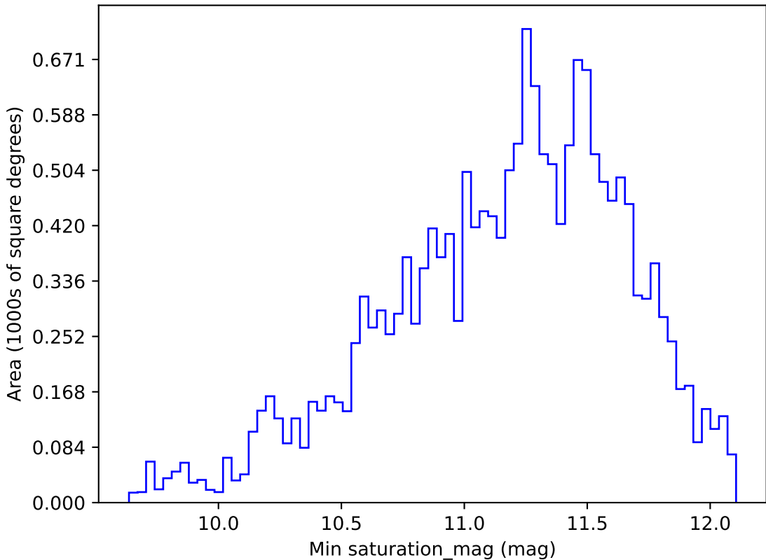
weather_cloudso12v3.4_10yrs WFD u band: Min saturation_mag
