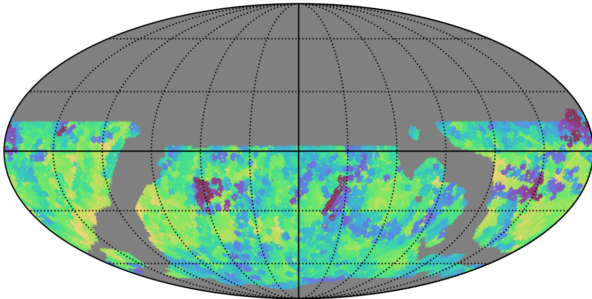
weather_cloudso12v3.4_10yrs WFD r band: Min saturation_mag
