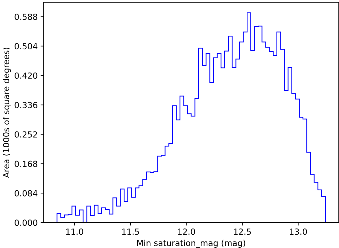
weather_cloudso12v3.4_10yrs WFD r band: Min saturation_mag
