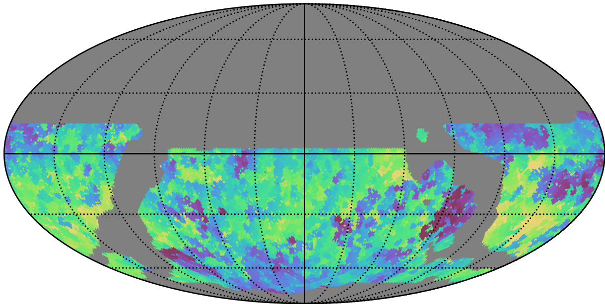
weather_cloudso12v3.4_10yrs WFD g band: Min saturation_mag
