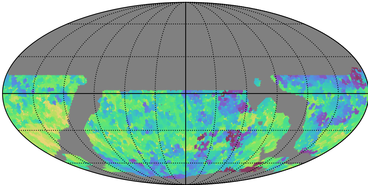
weather_cloudso12v3.4_10yrs WFD all bands: Min saturation_mag
