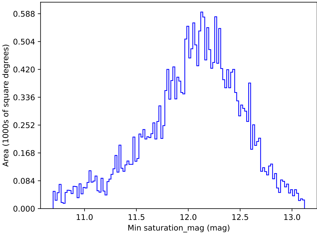
weather_cloudso12v3.4_10yrs All sky z band: Min saturation_mag
