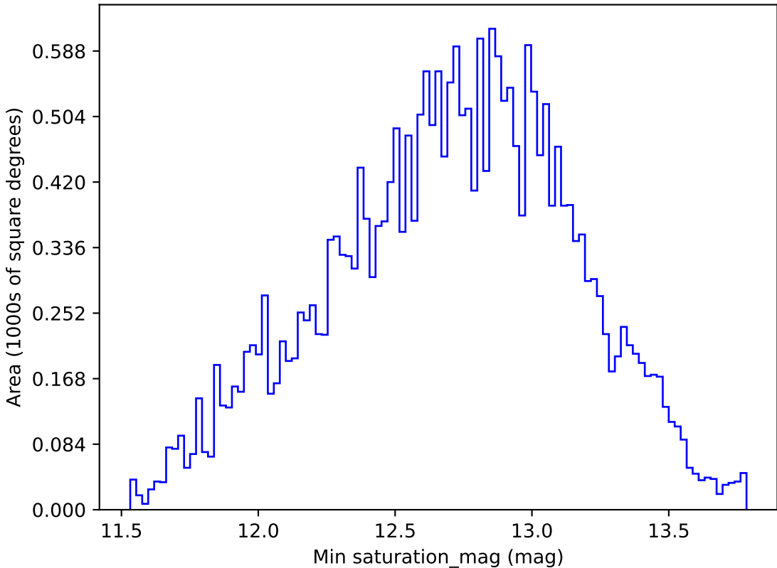
weather_cloudso12v3.4_10yrs All sky g band: Min saturation_mag
