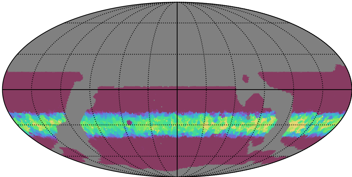
weather_cloudso12v3.4_10yrs WFD z band: Min normairmass
