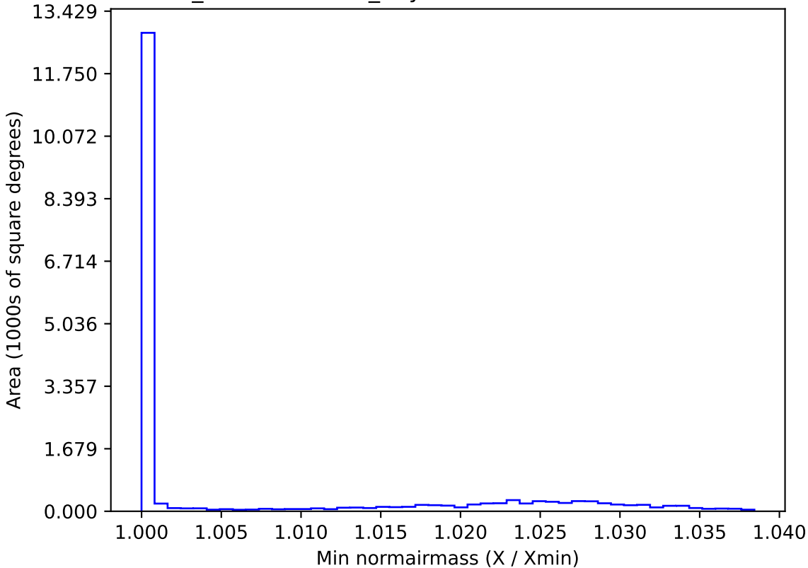
weather_cloudso12v3.4_10yrs WFD z band: Min normairmass
